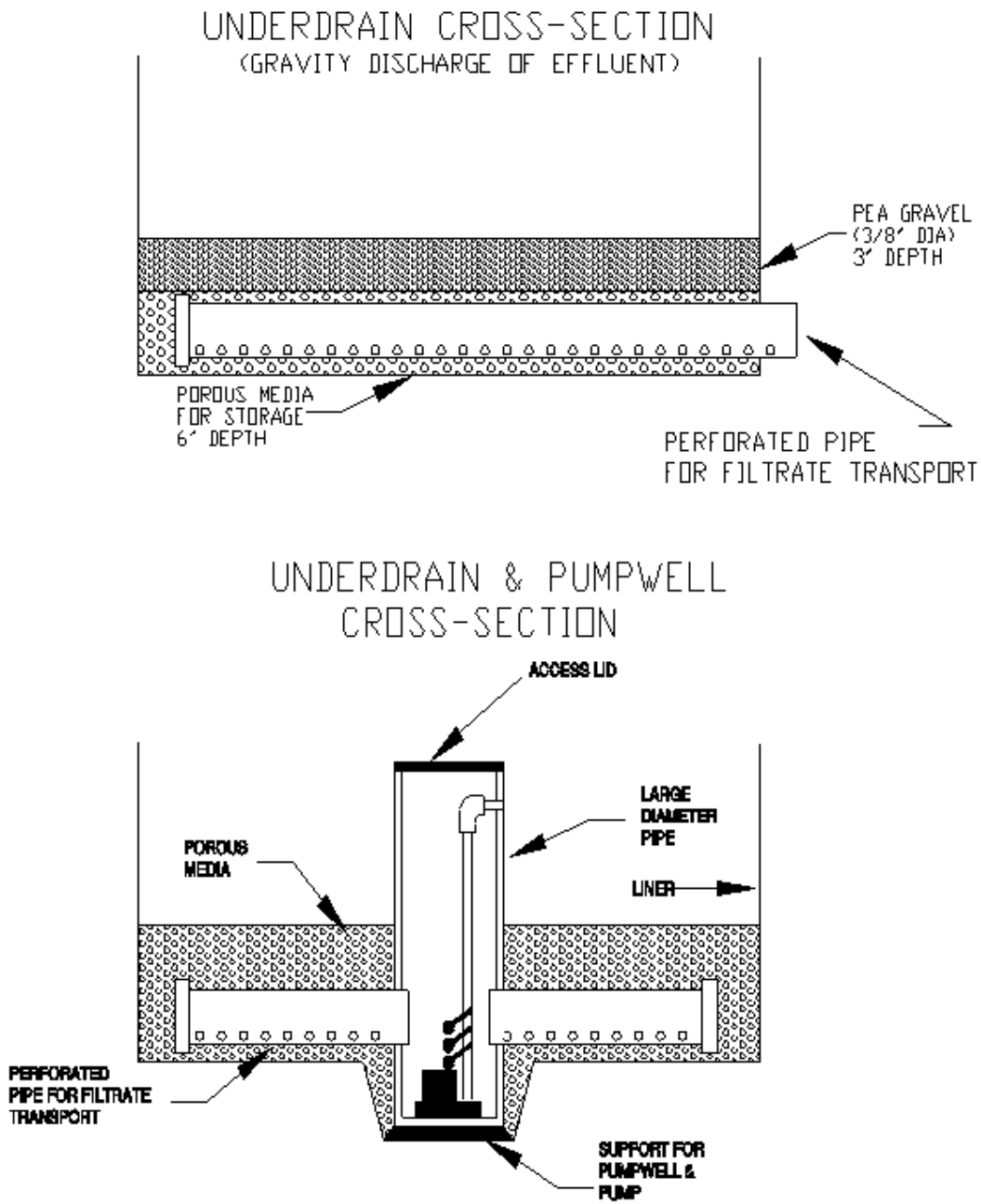
Figure 9 Intermittent Sand Filter Underdrain & Pumpwell
