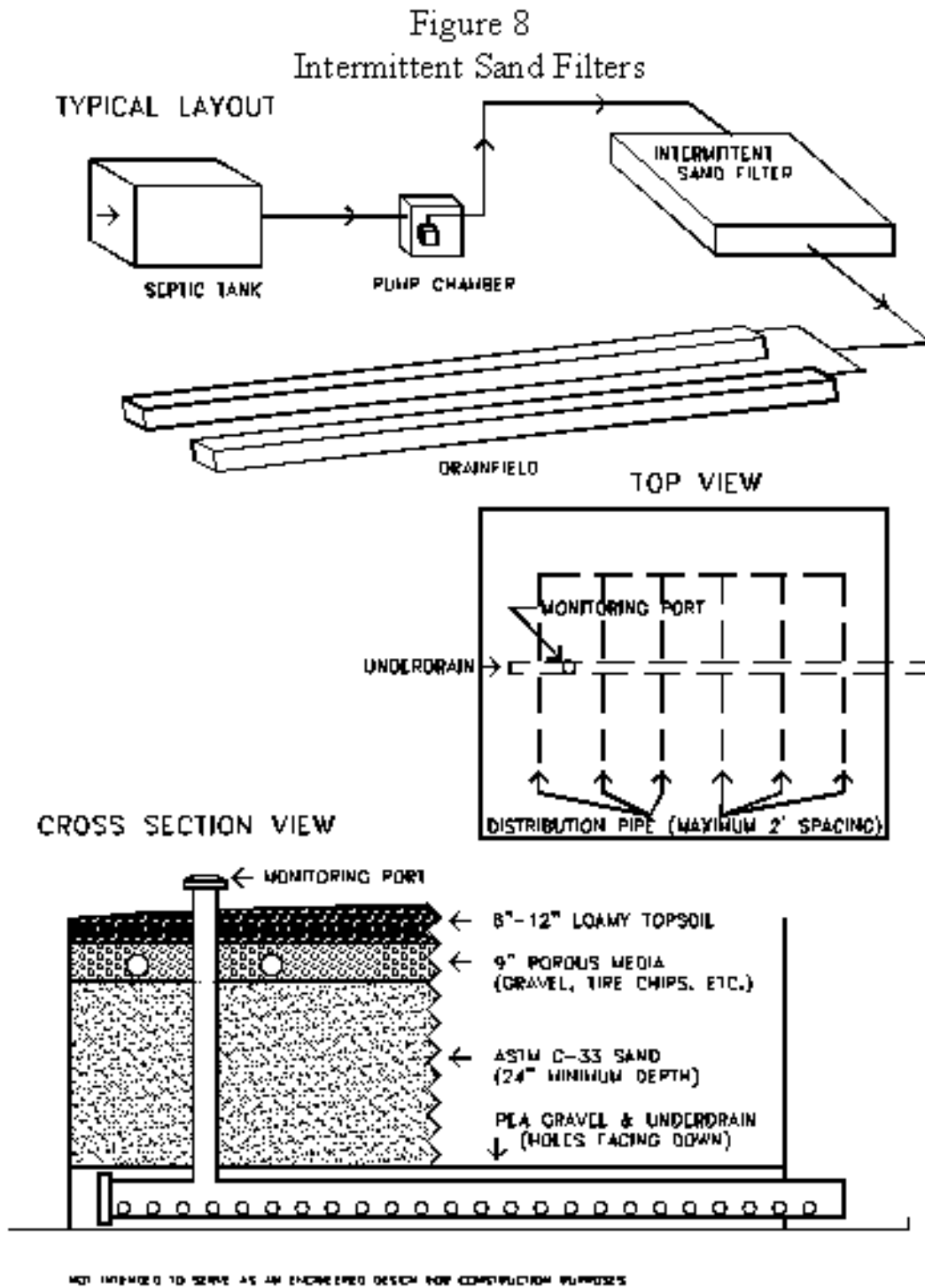
(8) Figure 8. Intermittent Sand Filters.
